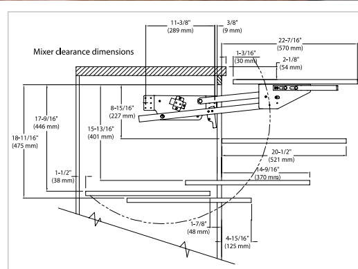
ML-WNHDSCOG-18FL Soft-Close Mixer Lift Kit (Walnut/Orion Gray finish shown)
